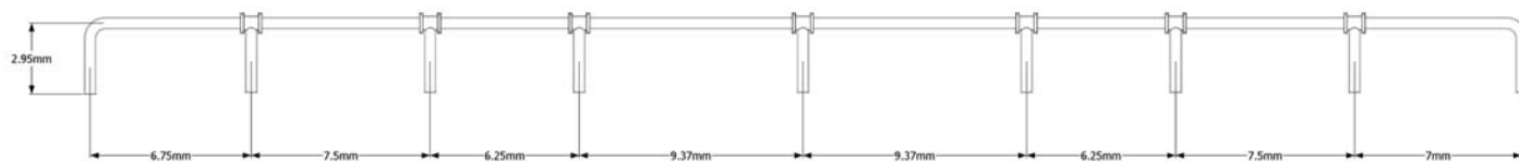
Main Top Grab Rail – 2 No. Required
