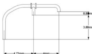
Outer Ladder Grab Rail 4 No. Required
