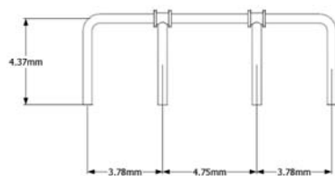
Top End Grab Rail 2 No. Required
