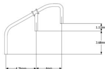
Inner Ladder Grab Rail 4 No. Required
